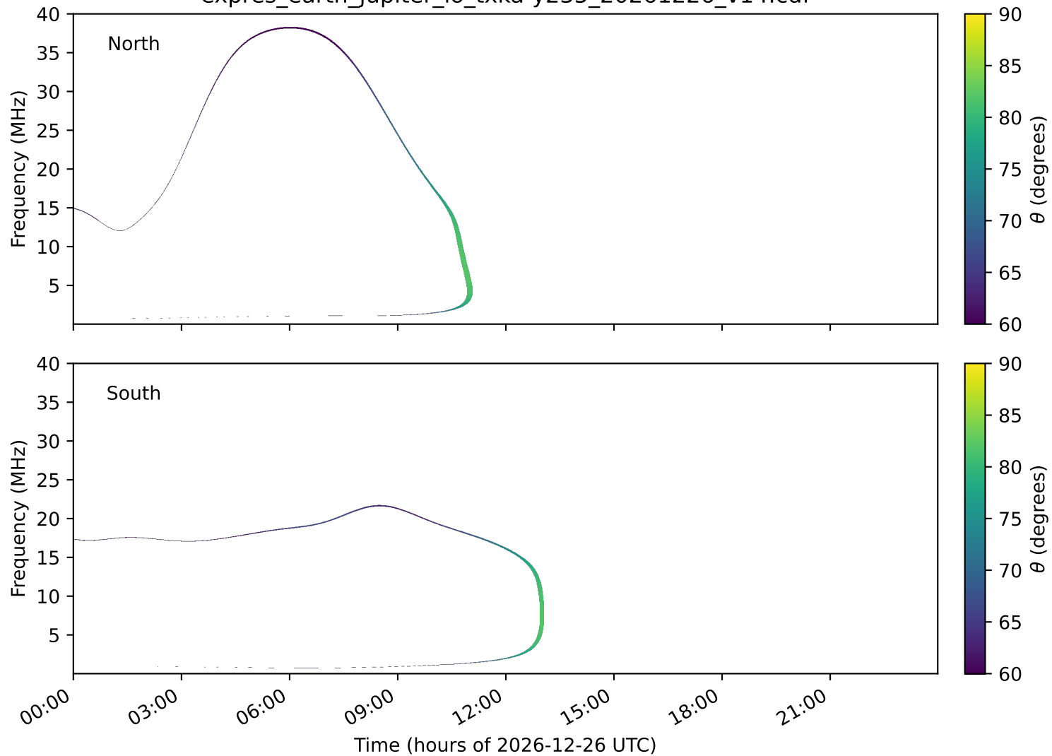
expres_earth_jupiter_io_txka-y235_20261226_v14.cdf
