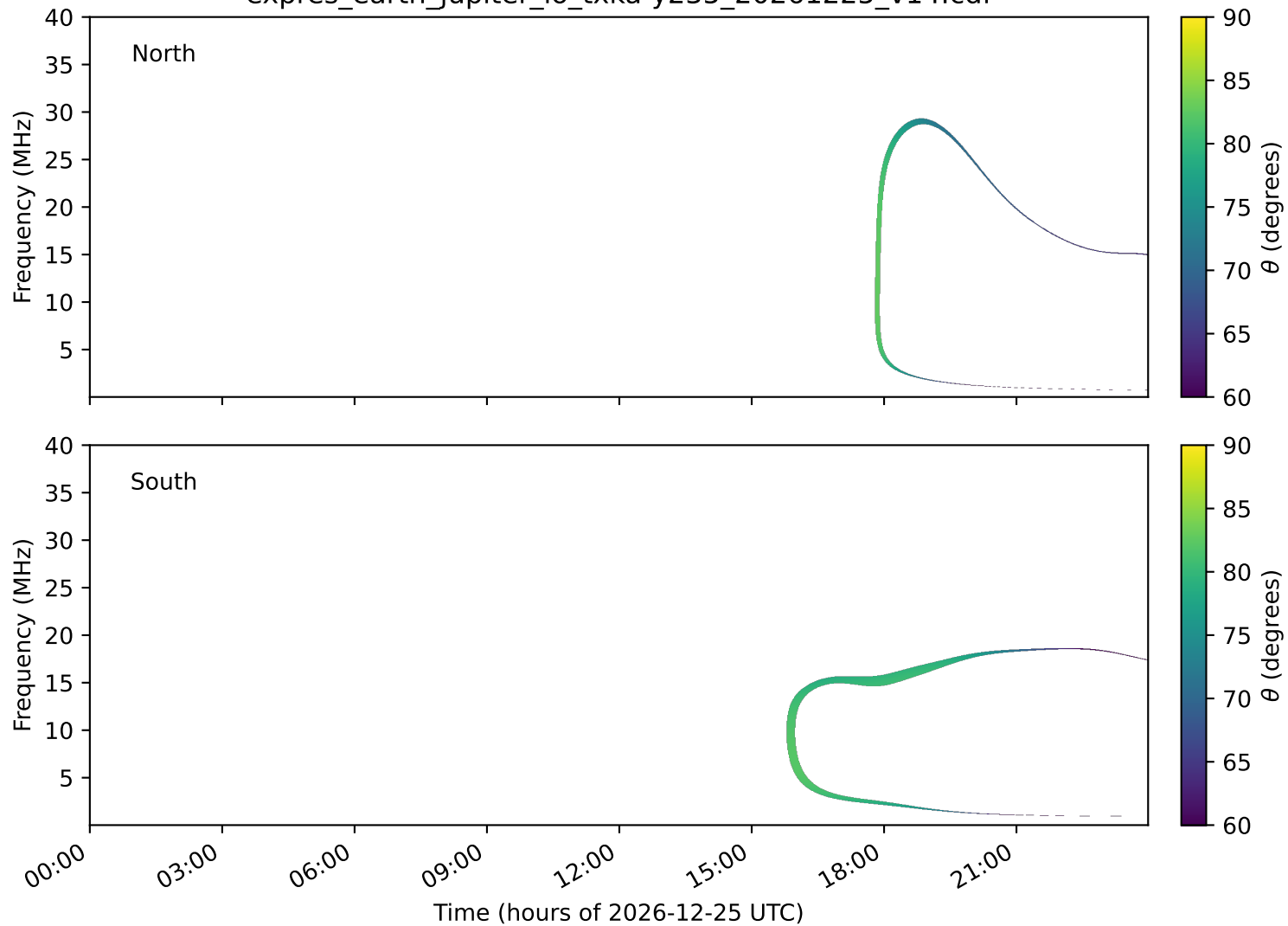
expres_earth_jupiter_io_txka-y235_20261225_v14.cdf
