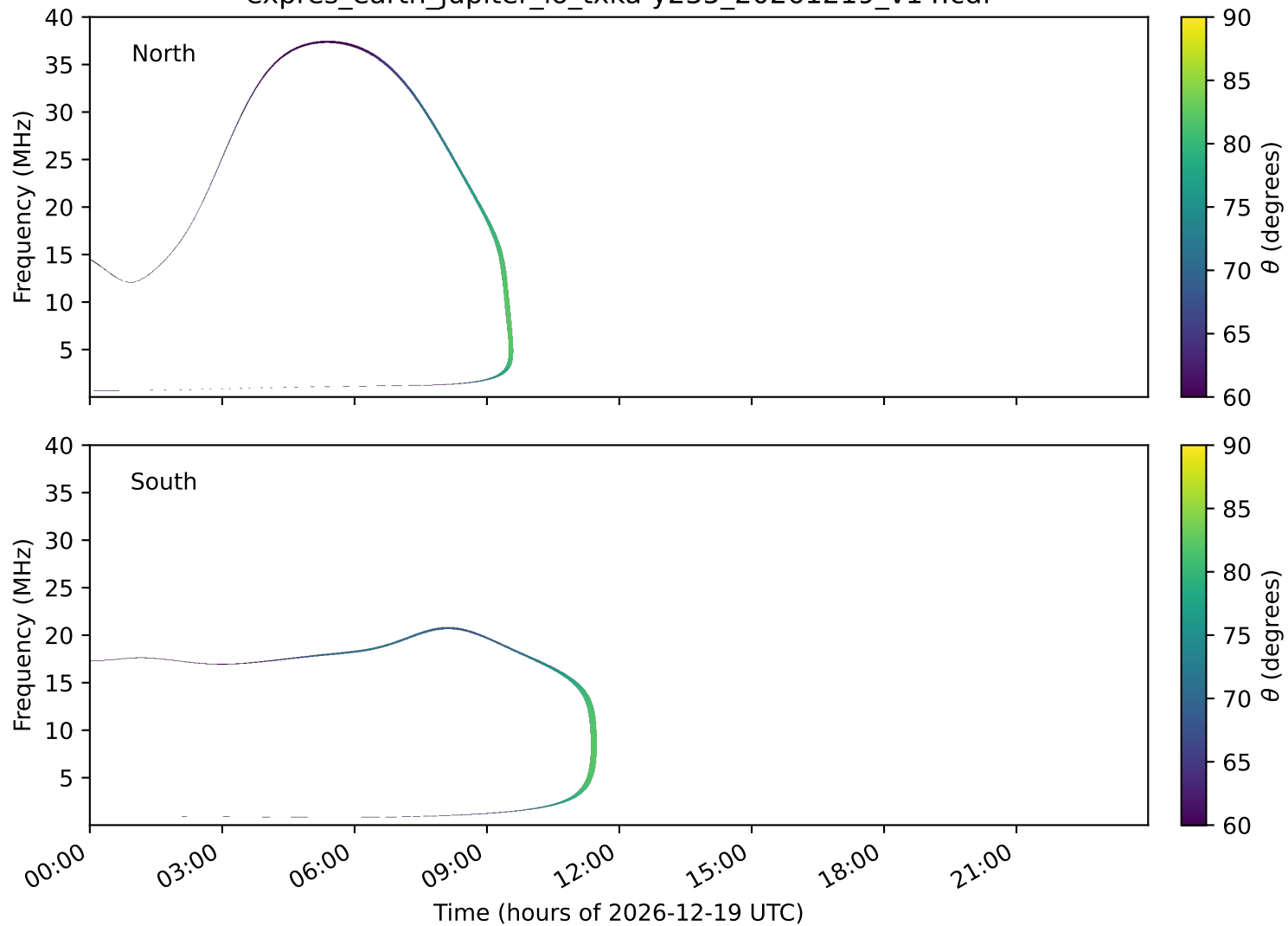
expres_earth_jupiter_io_txka-y235_20261219_v14.cdf
