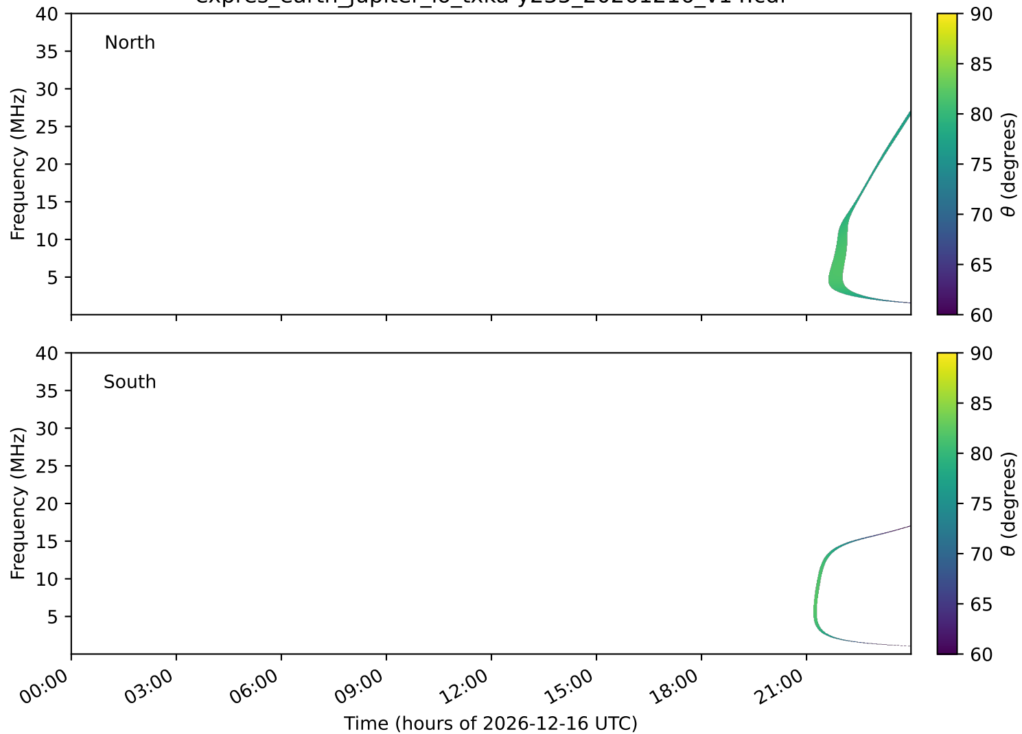
expres_earth_jupiter_io_txka-y235_20261216_v14.cdf
