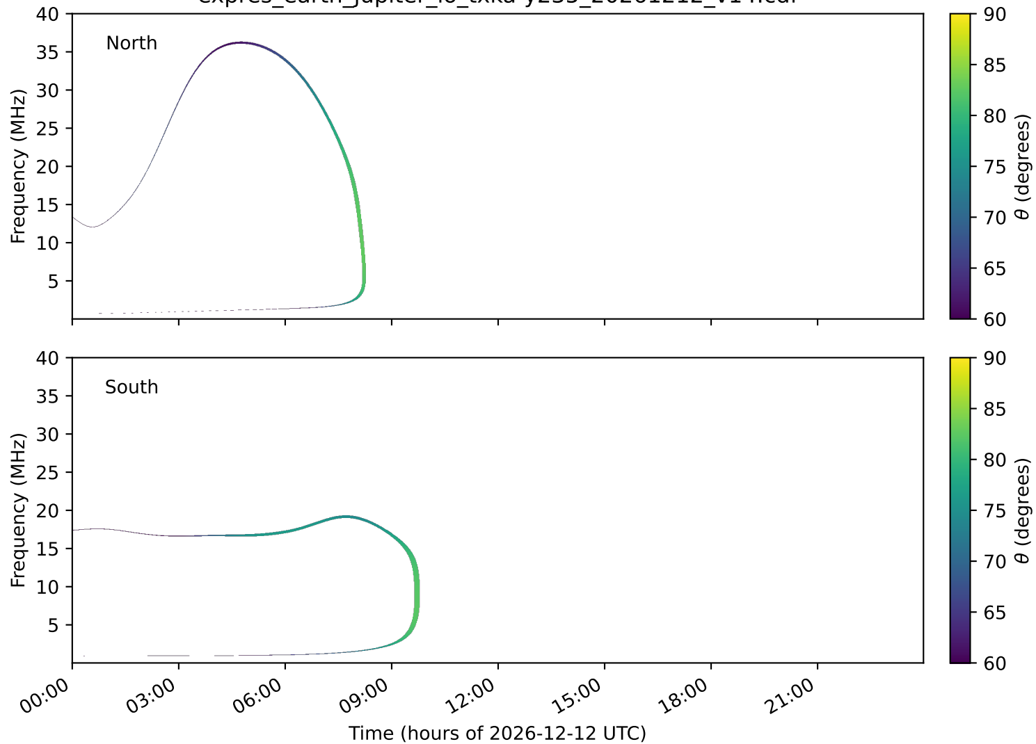
expres_earth_jupiter_io_txka-y235_20261212_v14.cdf
