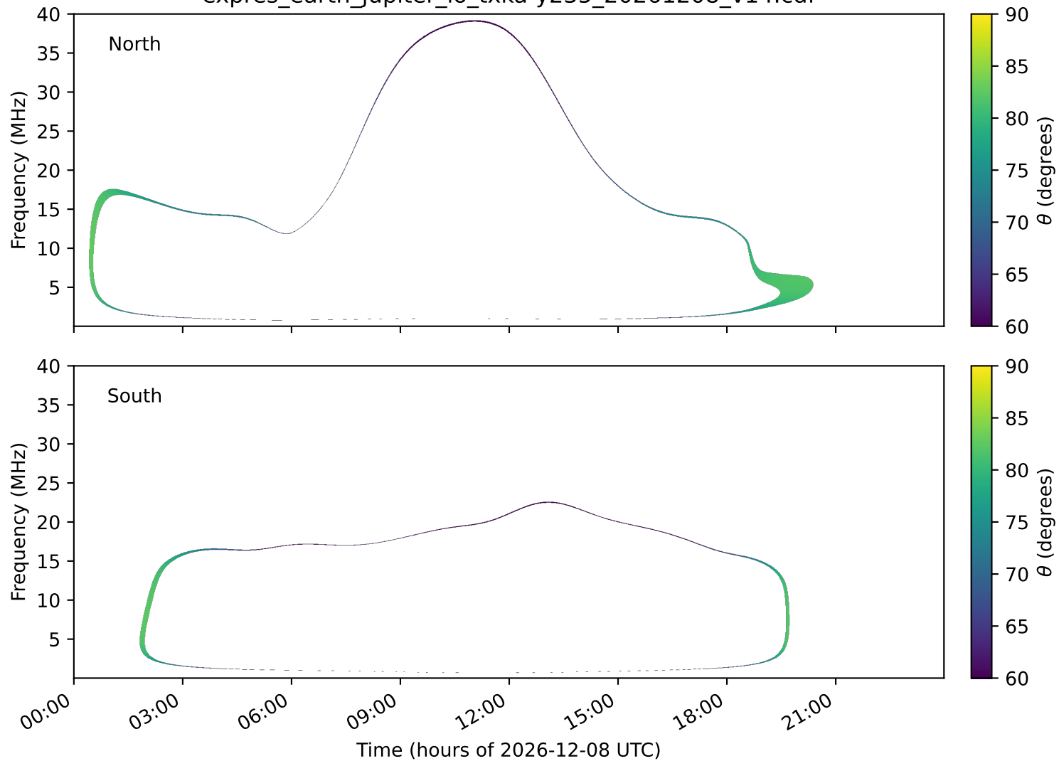
expres_earth_jupiter_io_txka-y235_20261208_v14.cdf
