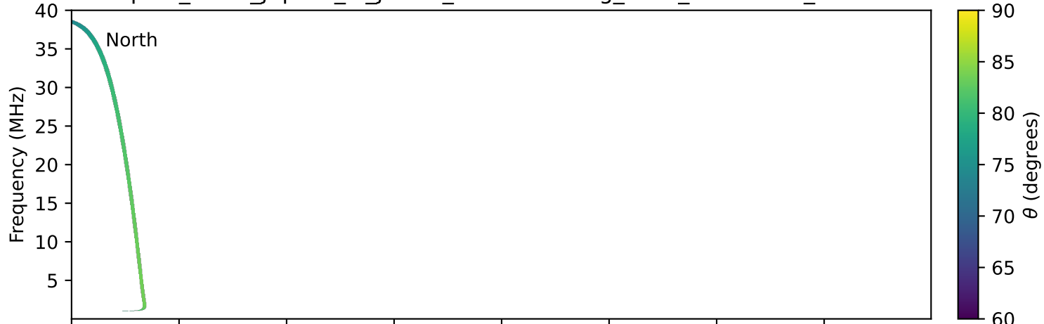
expres_earth_jupiter_io_jrm33_lossc-wid1deg_3kev_20261230_v11.cdf
