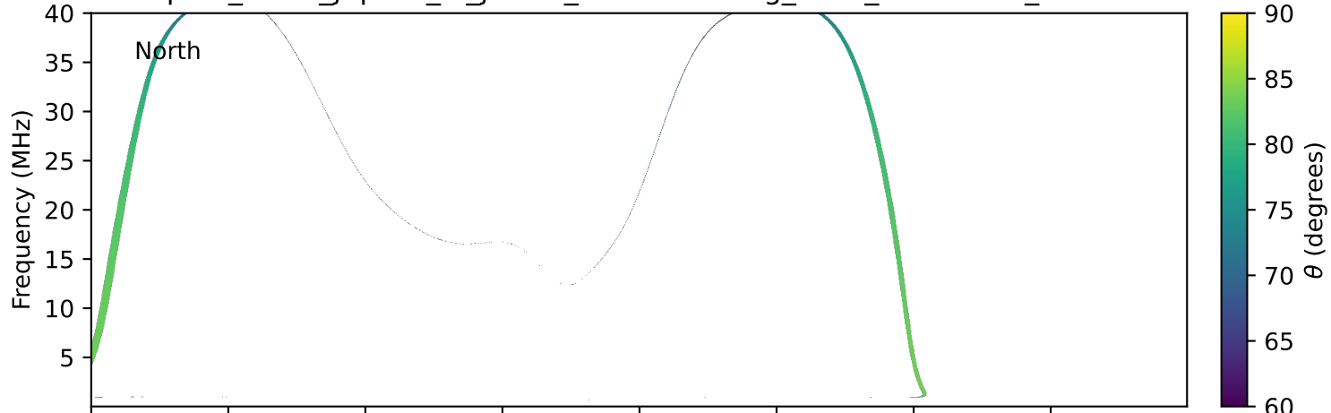
expres_earth_jupiter_io_jrm33_lossc-wid1deg_3kev_20261224_v11.cdf
