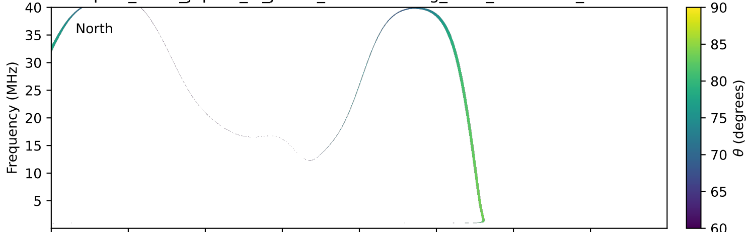
expres_earth_jupiter_io_jrm33_lossc-wid1deg_3kev_20261217_v11.cdf
