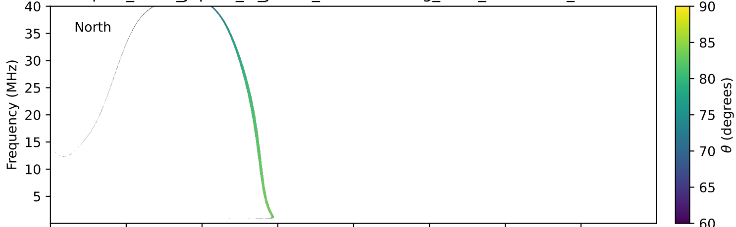
expres_earth_jupiter_io_jrm33_lossc-wid1deg_3kev_20261212_v11.cdf
