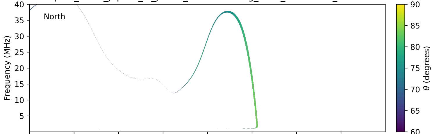
expres_earth_jupiter_io_jrm33_lossc-wid1deg_3kev_20261210_v11.cdf
