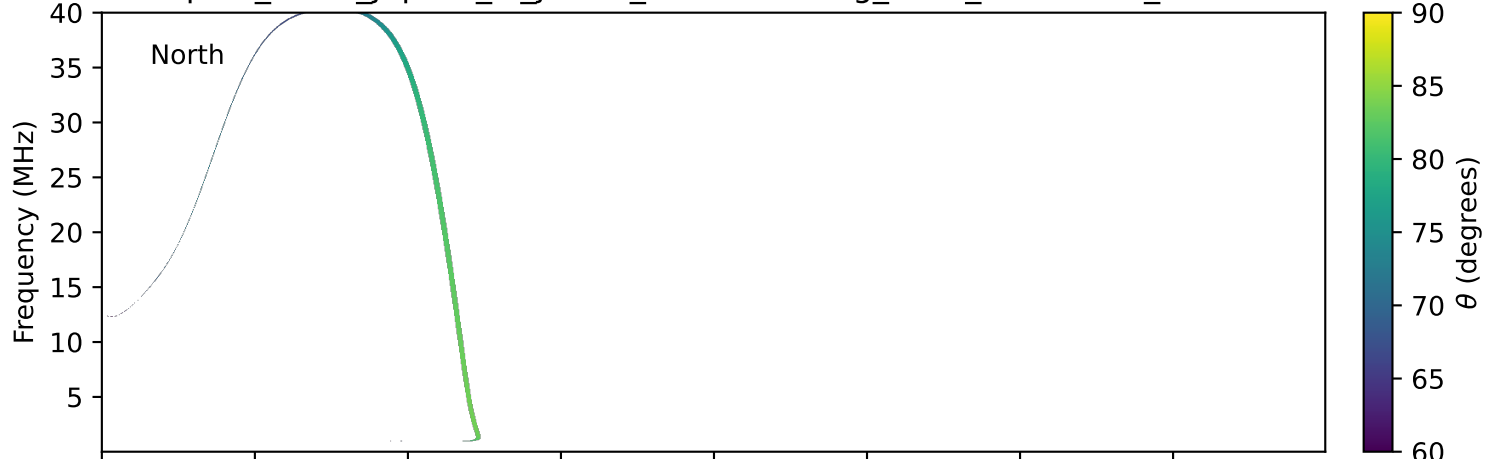
expres_earth_jupiter_io_jrm33_lossc-wid1deg_3kev_20261205_v11.cdf
