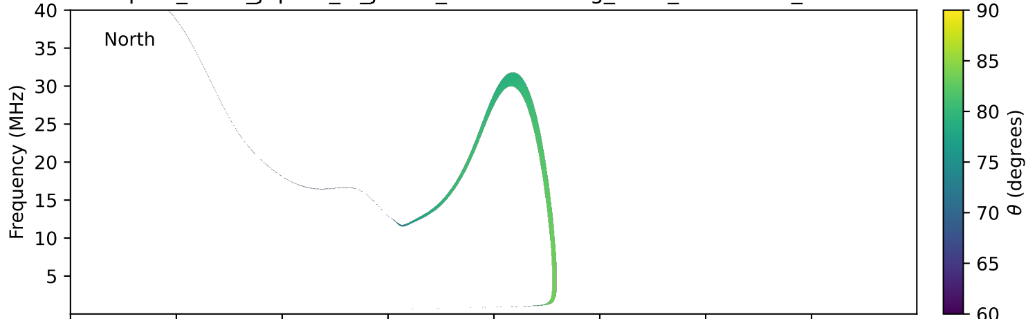
expres_earth_jupiter_io_jrm33_lossc-wid1deg_3kev_20261203_v11.cdf
