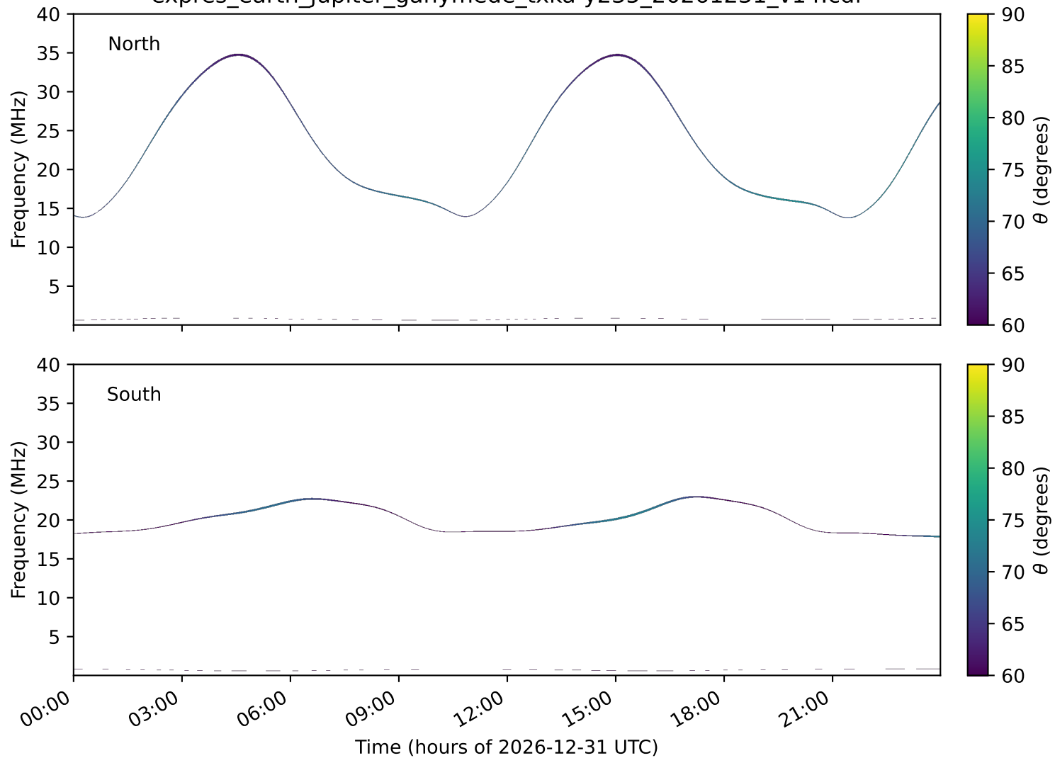
expres_earth_jupiter_ganymede_txka-y235_20261231_v14.cdf
