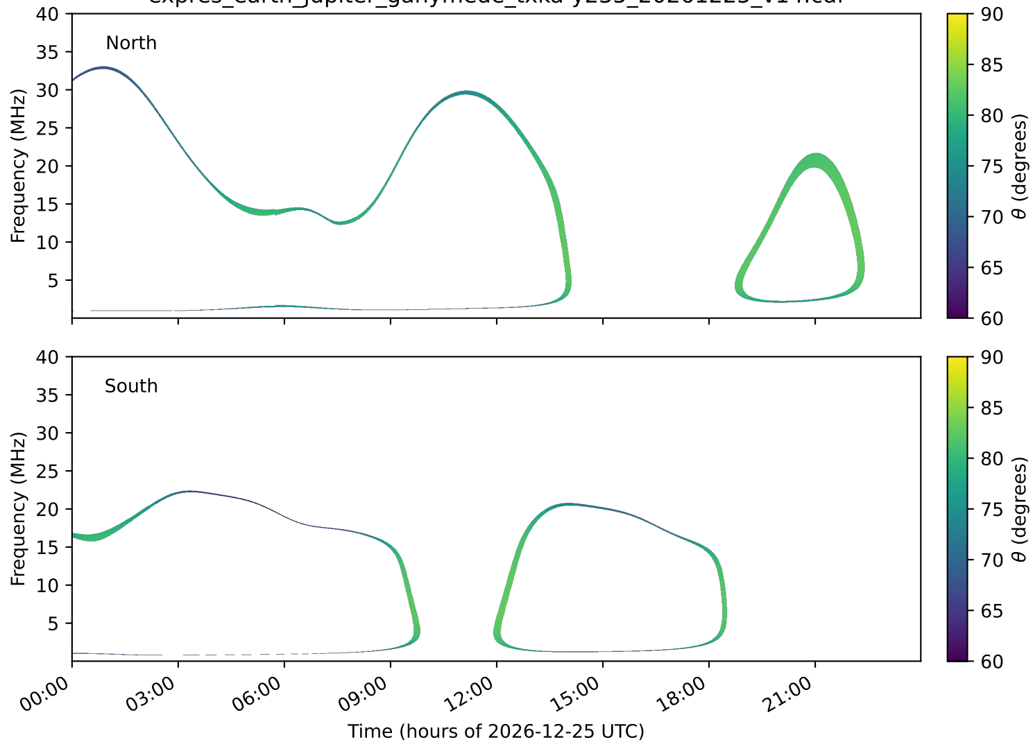
expres_earth_jupiter_ganymede_txka-y235_20261225_v14.cdf
