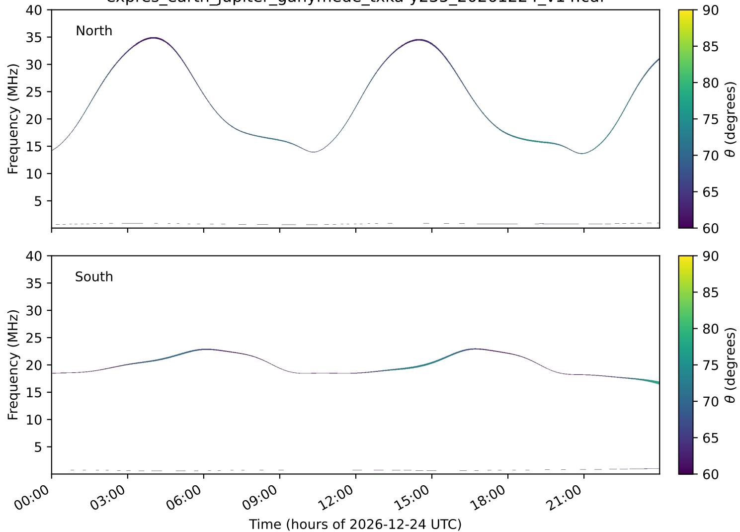
expres_earth_jupiter_ganymede_txka-y235_20261224_v14.cdf
