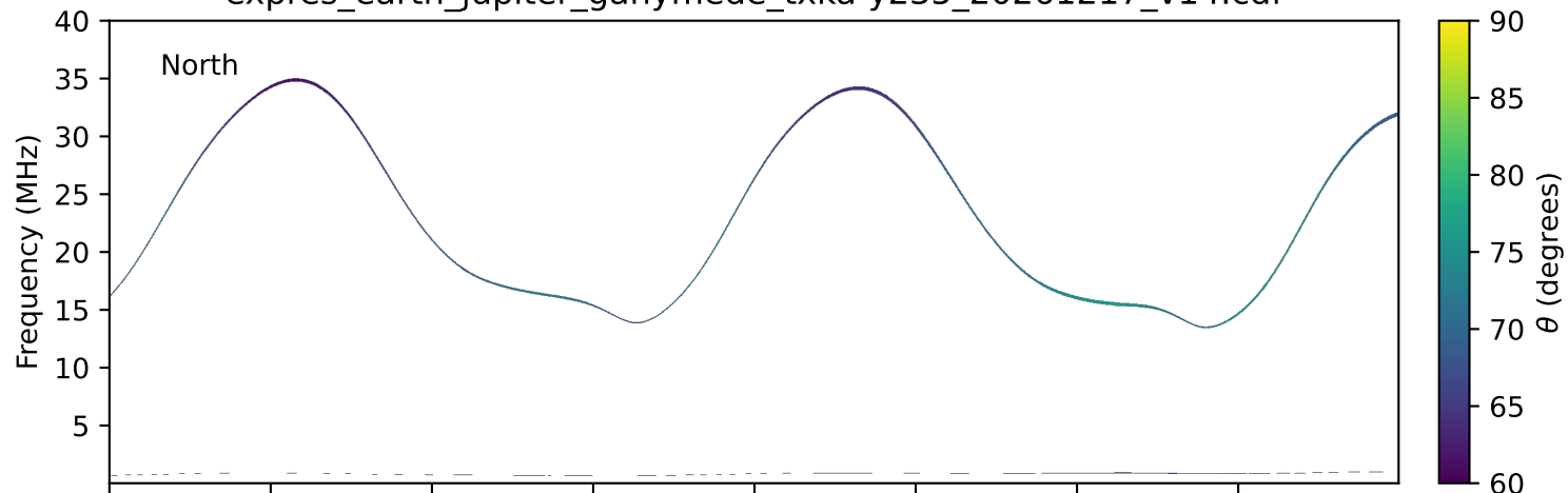
expres_earth_jupiter_ganymede_txka-y235_20261217_v14.cdf
