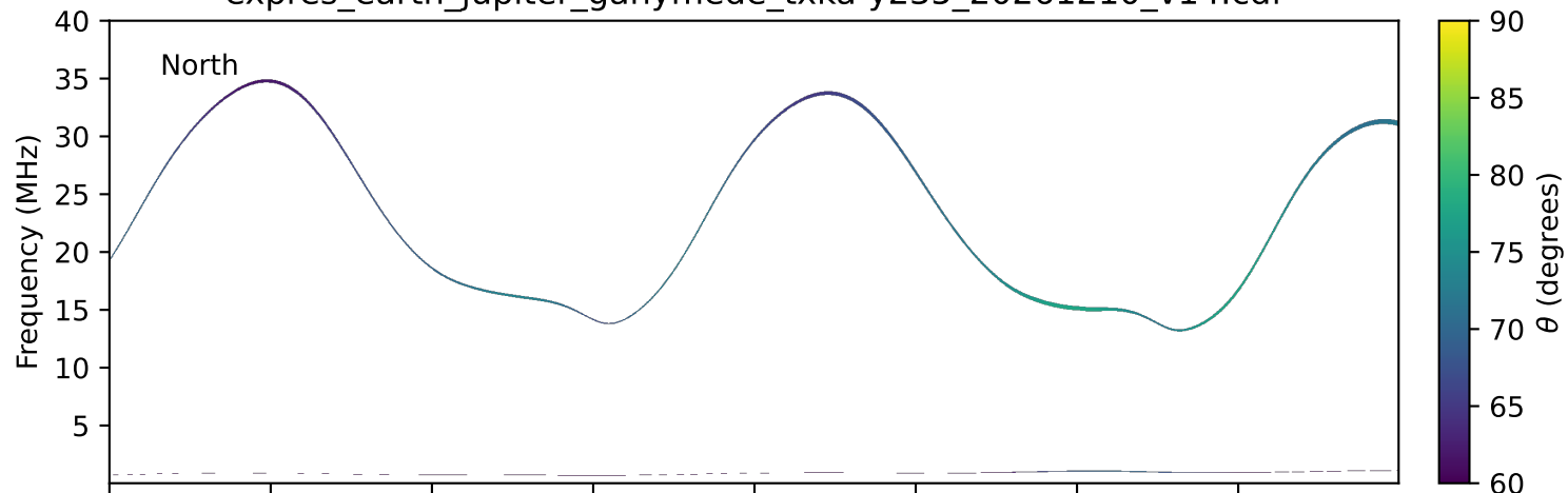
expres_earth_jupiter_ganymede_txka-y235_20261210_v14.cdf
