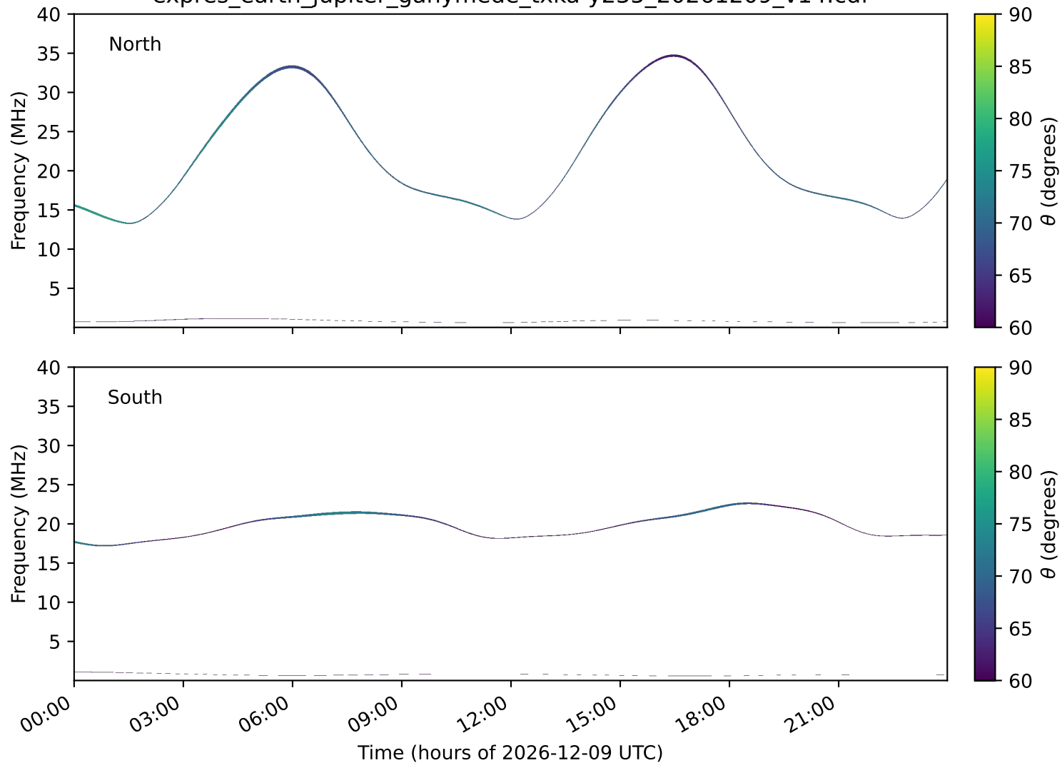
expres_earth_jupiter_ganymede_txka-y235_20261209_v14.cdf
