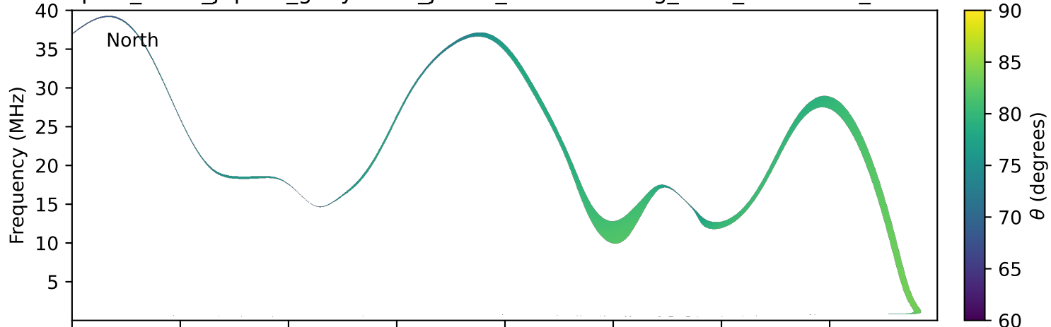
expres_earth_jupiter_ganymede_jrm33_lossc-wid1deg_3kev_20261225_v11.cdf
