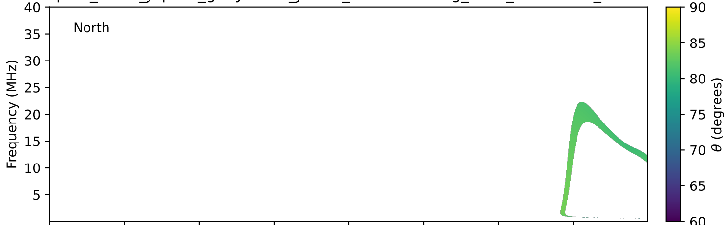
expres_earth_jupiter_ganymede_jrm33_lossc-wid1deg_3kev_20261222_v11.cdf
