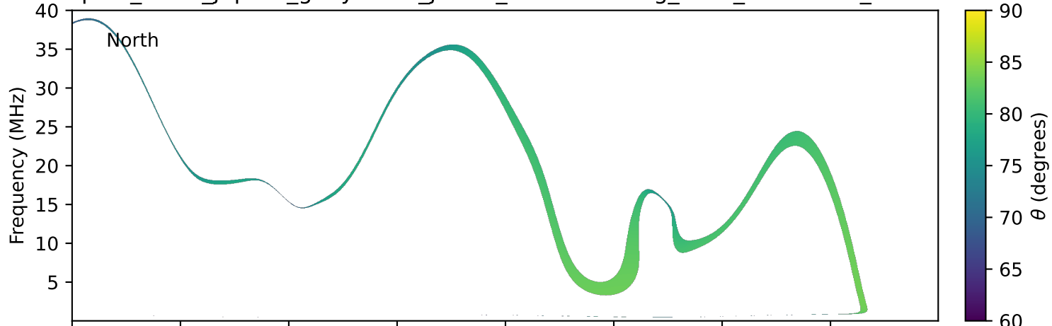
expres_earth_jupiter_ganymede_jrm33_lossc-wid1deg_3kev_20261218_v11.cdf
