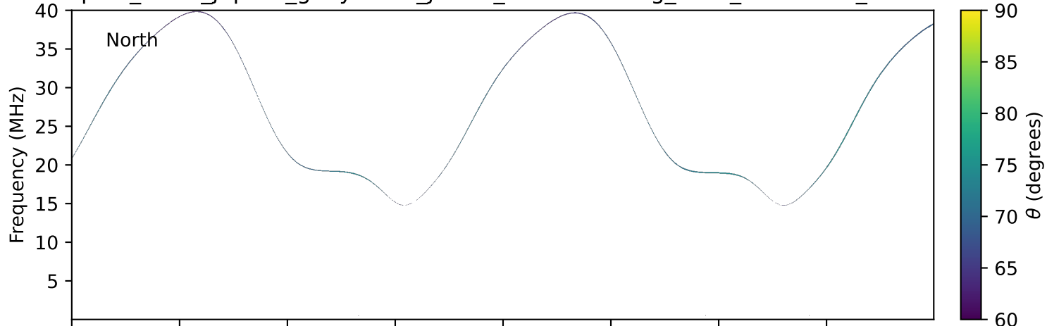
expres_earth_jupiter_ganymede_jrm33_lossc-wid1deg_3kev_20261217_v11.cdf
