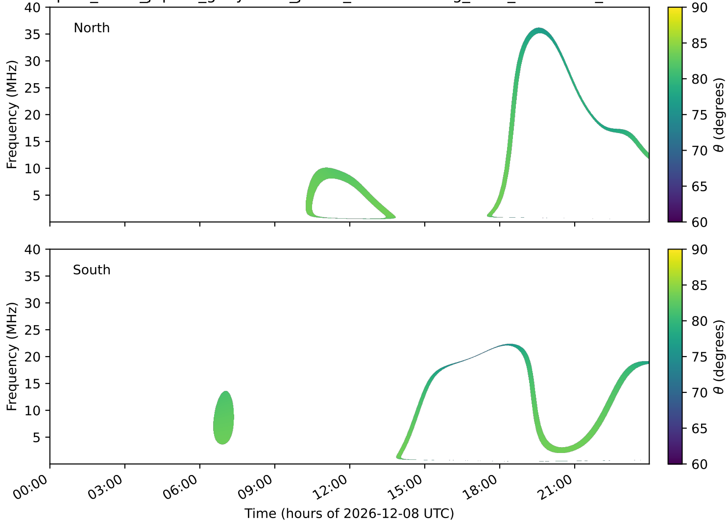
expres_earth_jupiter_ganymede_jrm33_lossc-wid1deg_3kev_20261208_v11.cdf
