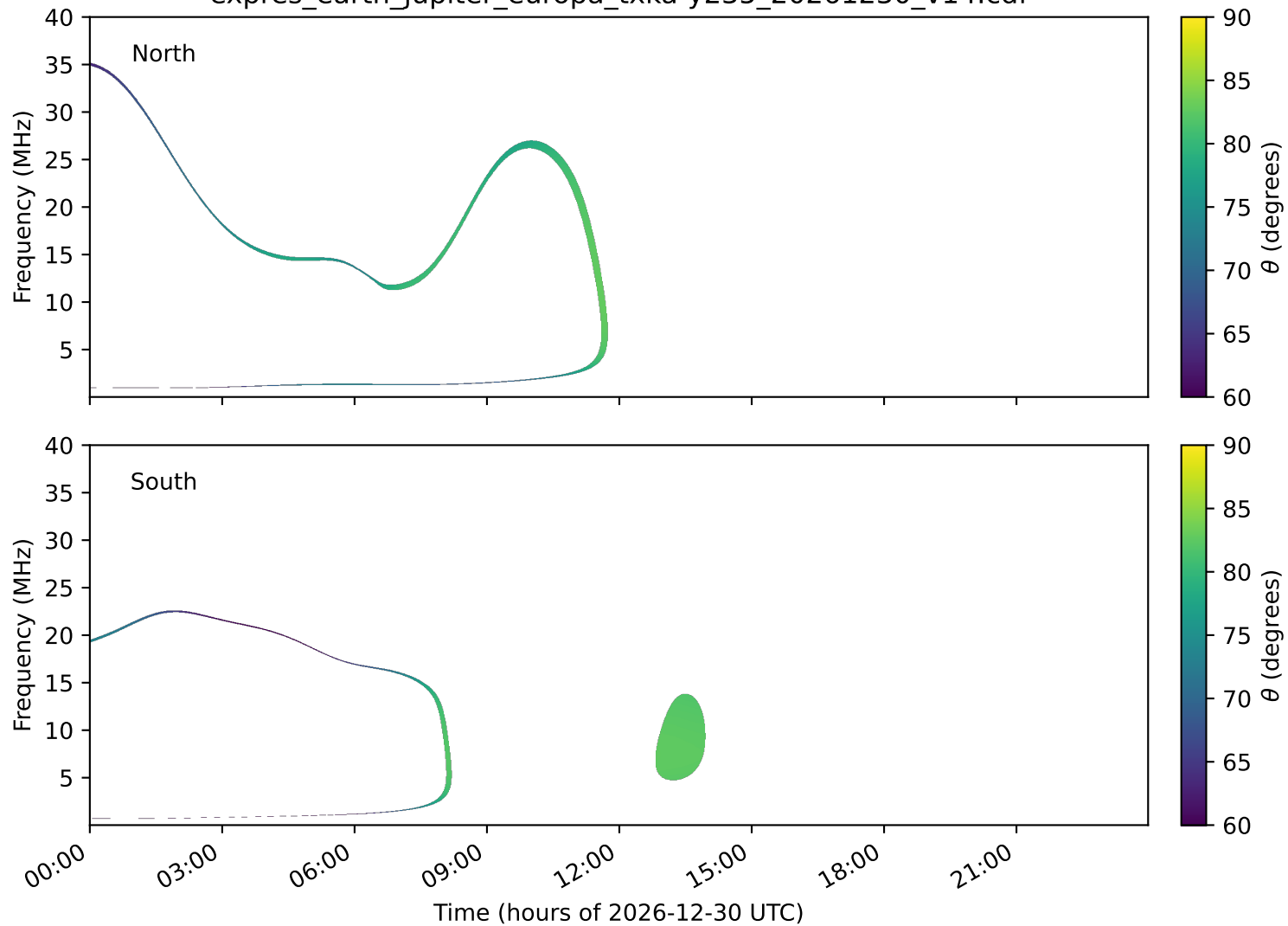
expres_earth_jupiter_europa_txka-y235_20261230_v14.cdf
