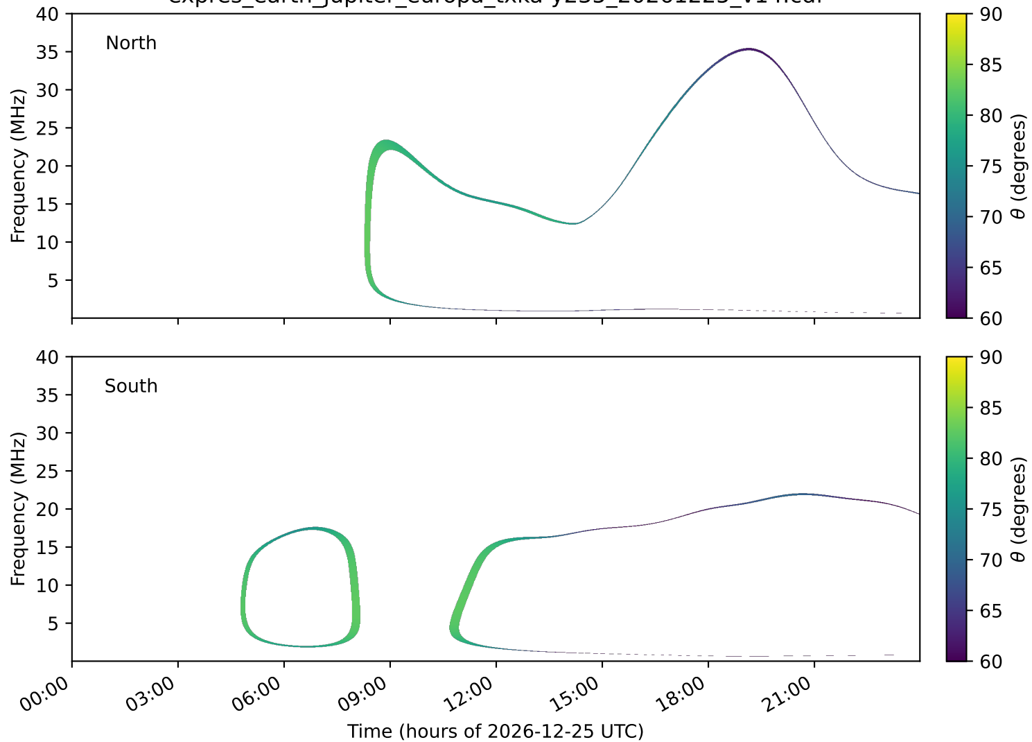
expres_earth_jupiter_europa_txka-y235_20261225_v14.cdf
