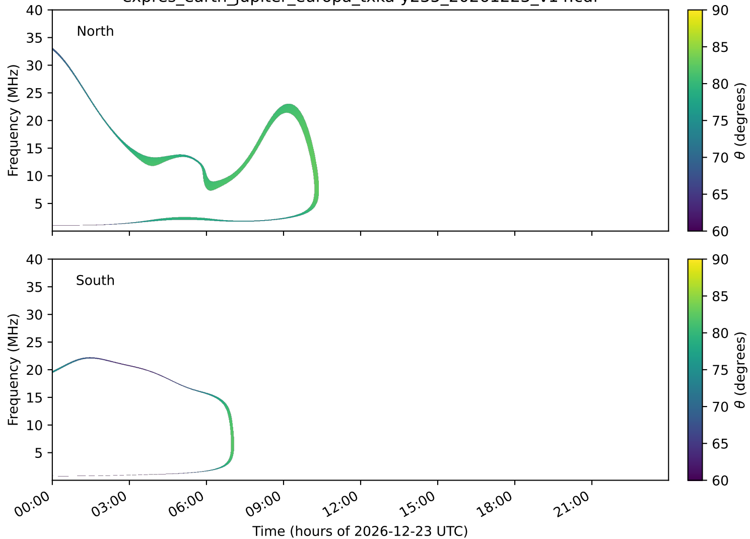
expres_earth_jupiter_europa_txka-y235_20261223_v14.cdf
