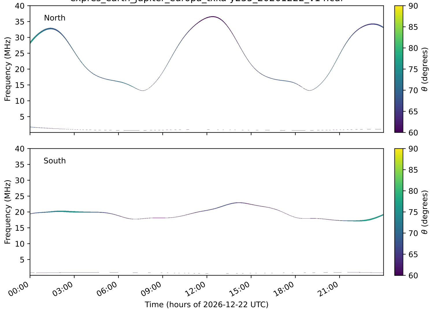
expres_earth_jupiter_europa_txka-y235_20261222_v14.cdf
