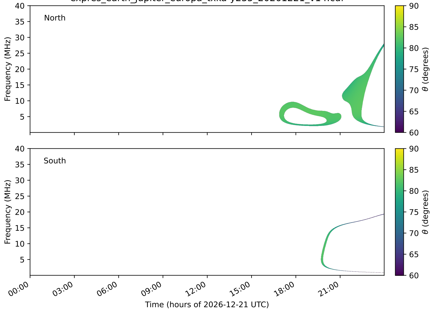
expres_earth_jupiter_europa_txka-y235_20261221_v14.cdf
