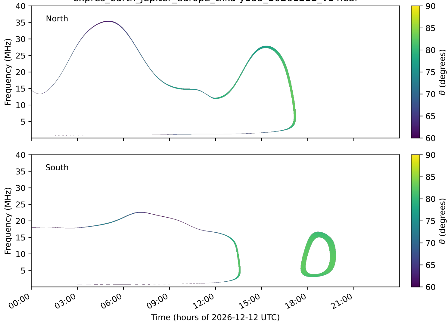
expres_earth_jupiter_europa_txka-y235_20261212_v14.cdf
