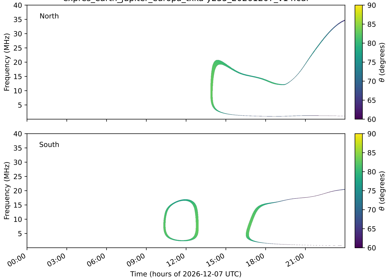
expres_earth_jupiter_europa_txka-y235_20261207_v14.cdf
