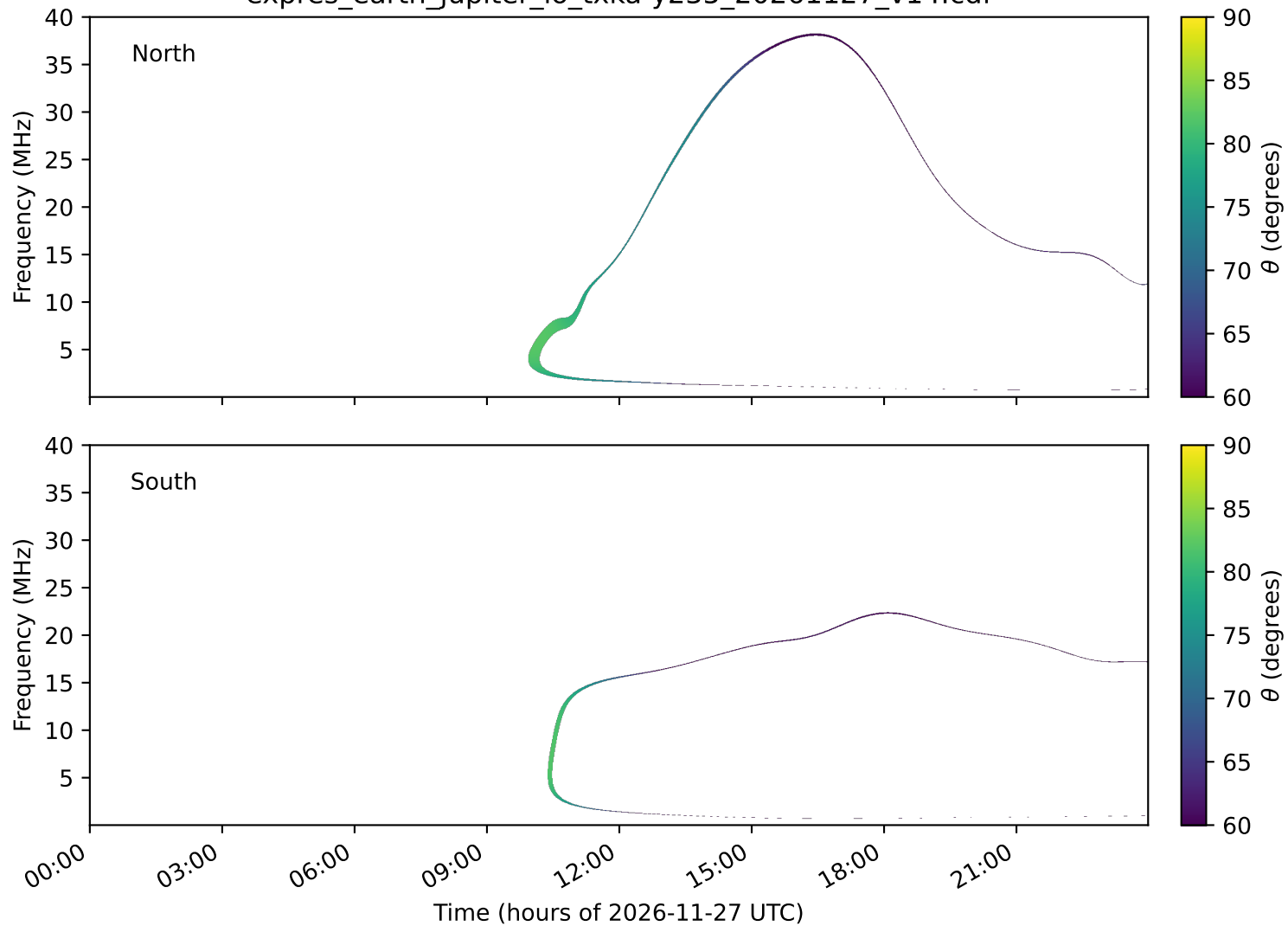
expres_earth_jupiter_io_txka-y235_20261127_v14.cdf
