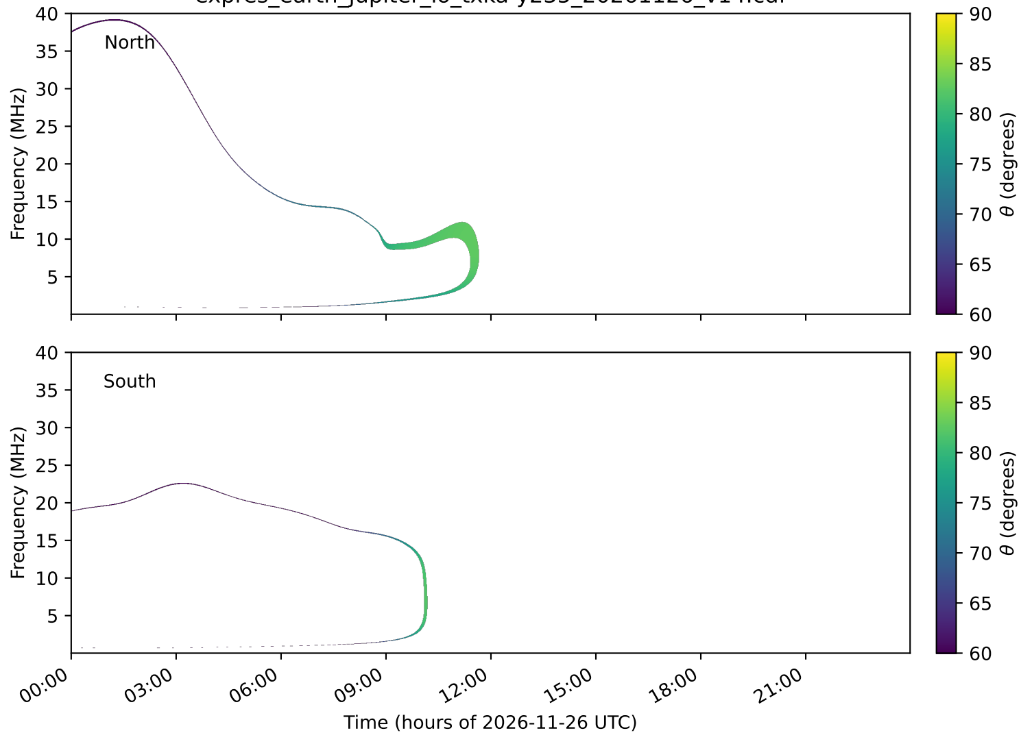
expres_earth_jupiter_io_txka-y235_20261126_v14.cdf
