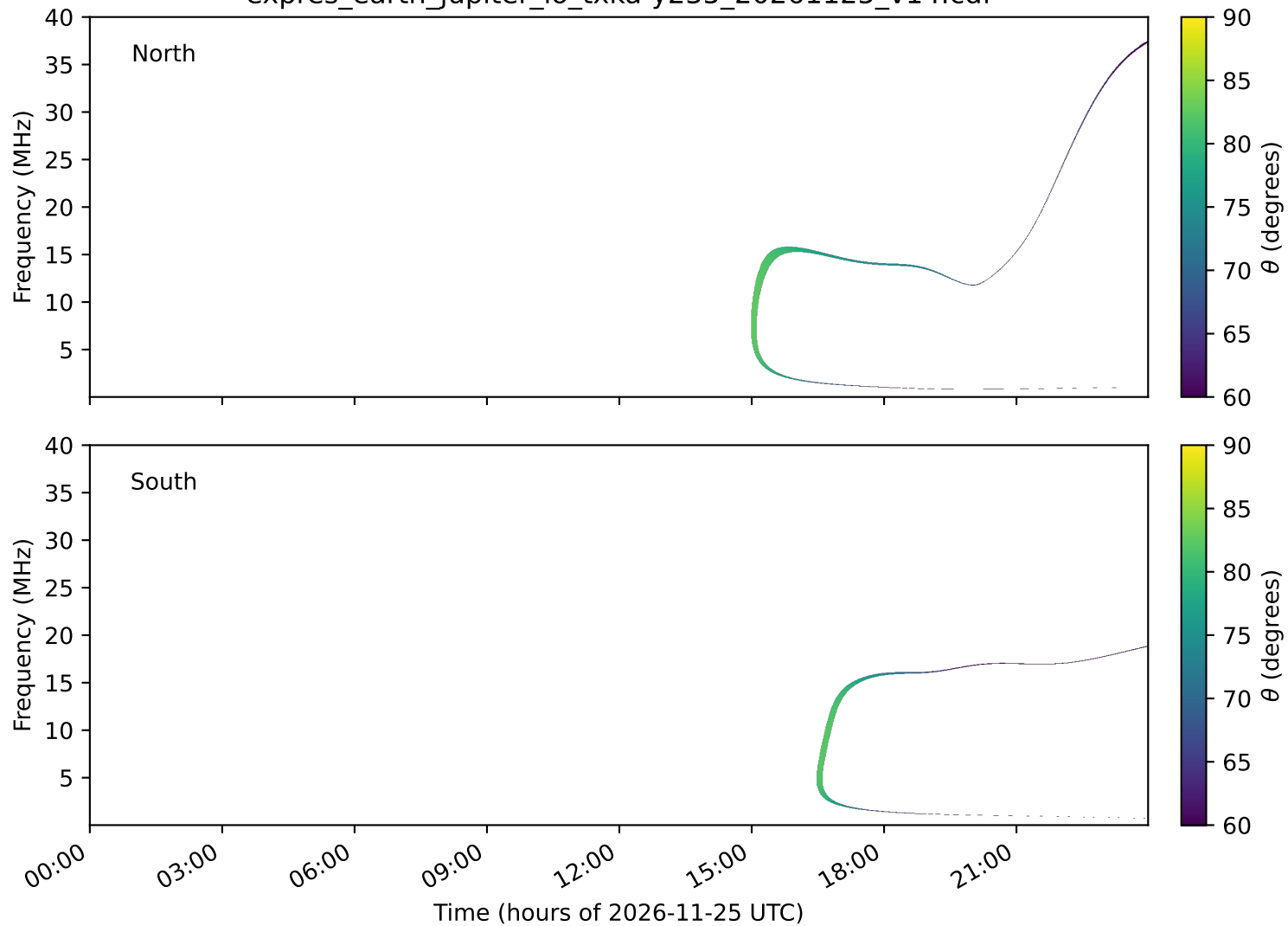
expres_earth_jupiter_io_txka-y235_20261125_v14.cdf
