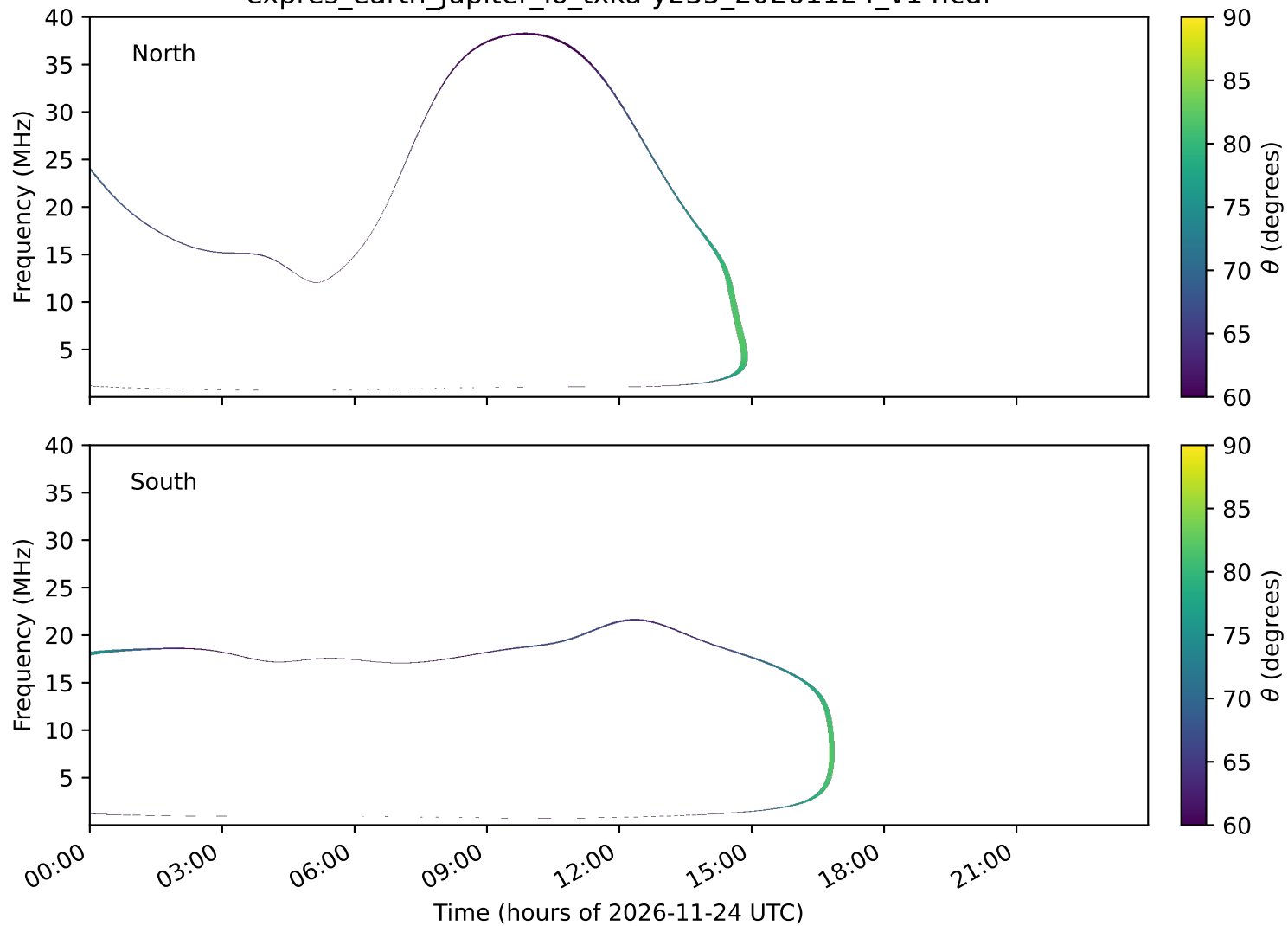
expres_earth_jupiter_io_txka-y235_20261124_v14.cdf
