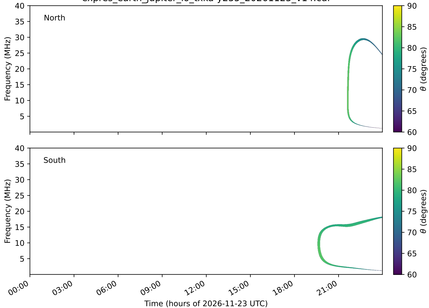
expres_earth_jupiter_io_txka-y235_20261123_v14.cdf
