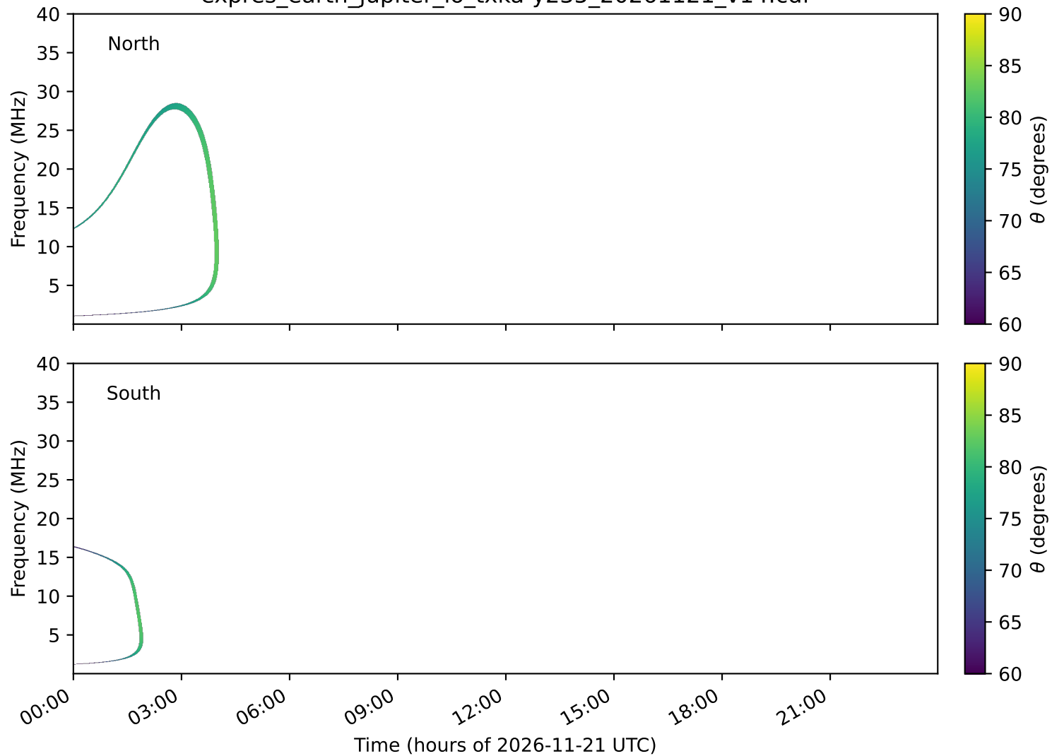
expres_earth_jupiter_io_txka-y235_20261121_v14.cdf
