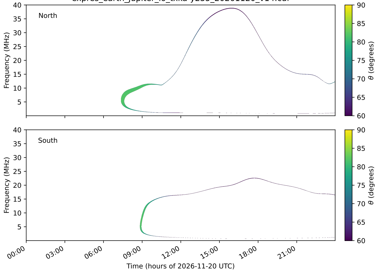
expres_earth_jupiter_io_txka-y235_20261120_v14.cdf
