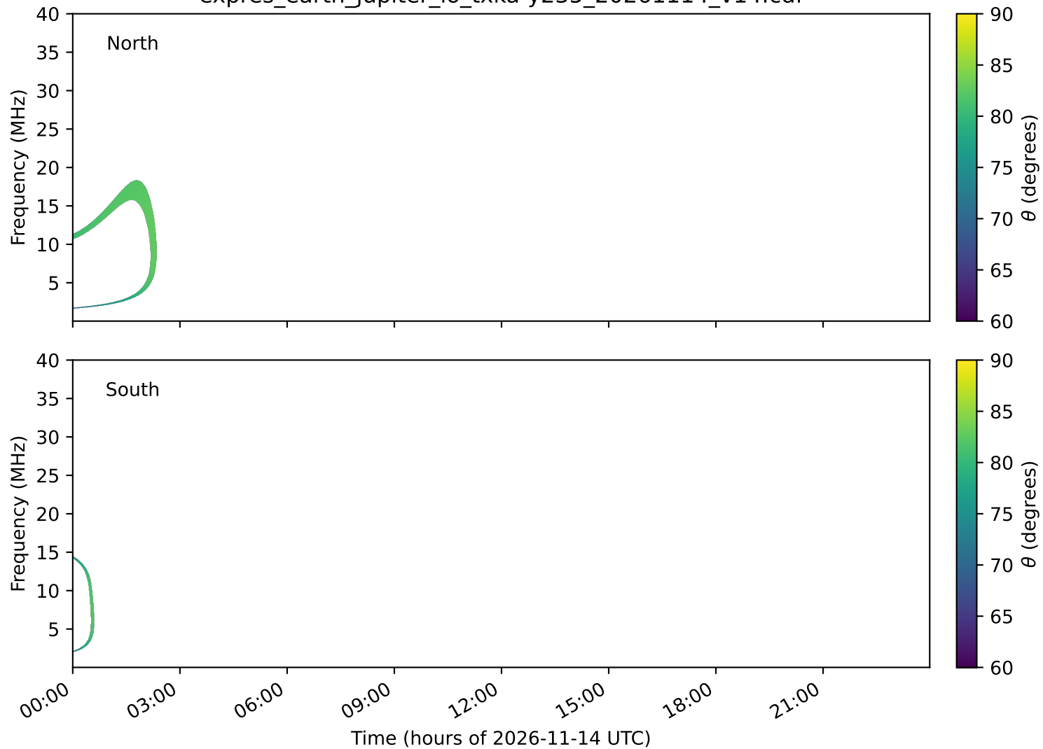
expres_earth_jupiter_io_txka-y235_20261114_v14.cdf
