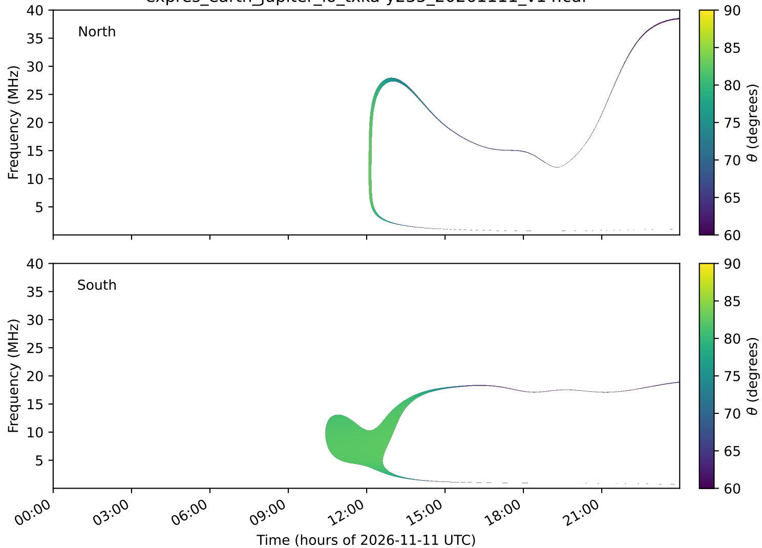
expres_earth_jupiter_io_txka-y235_20261111_v14.cdf
