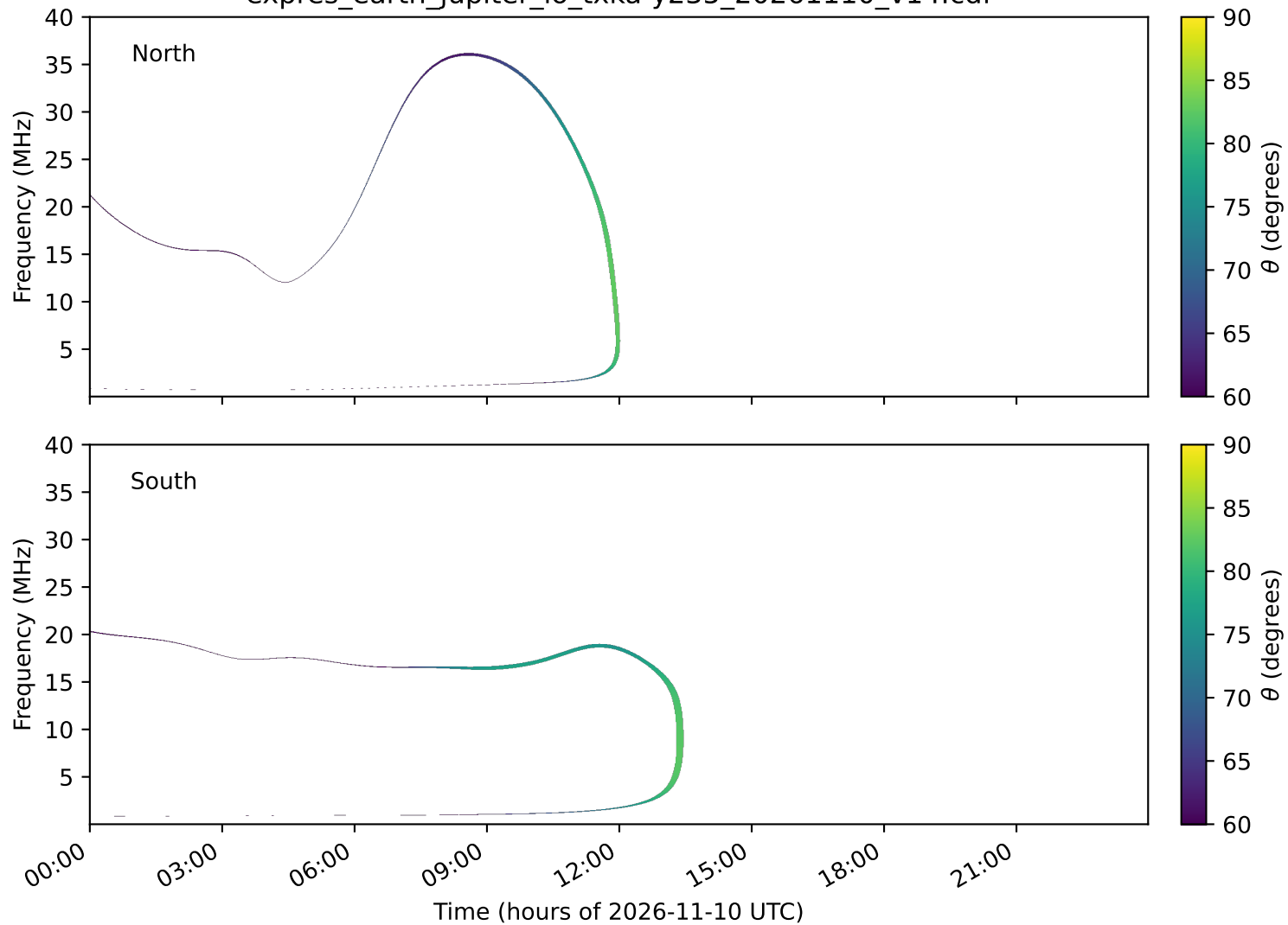
expres_earth_jupiter_io_txka-y235_20261110_v14.cdf
