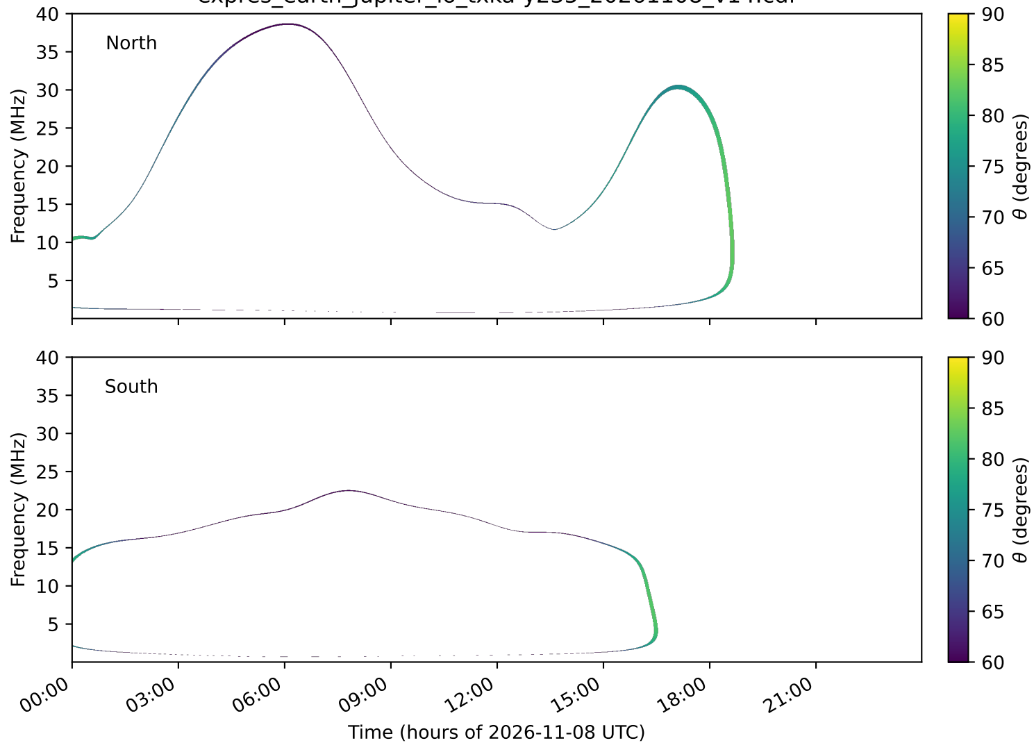
expres_earth_jupiter_io_txka-y235_20261108_v14.cdf
