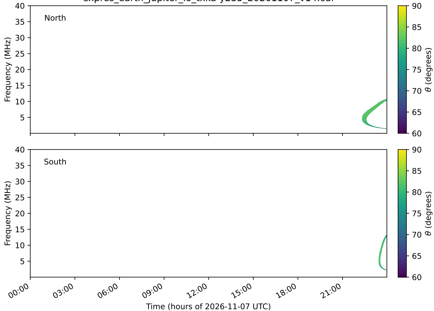
expres_earth_jupiter_io_txka-y235_20261107_v14.cdf
