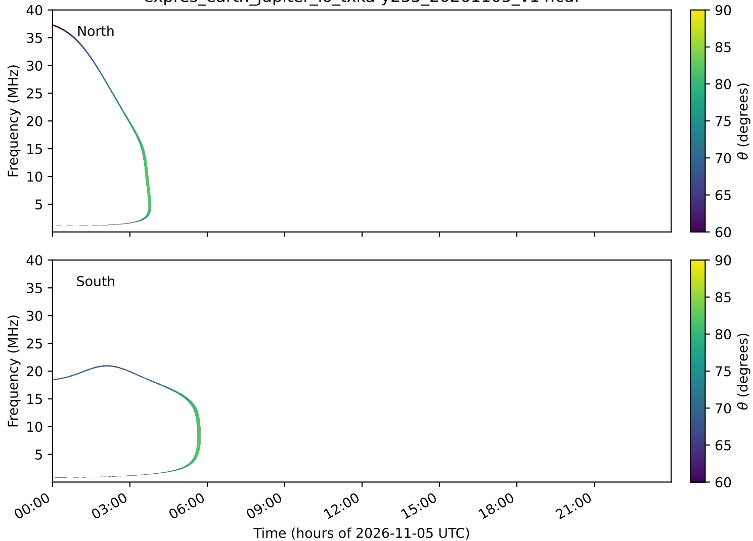
expres_earth_jupiter_io_txka-y235_20261105_v14.cdf
