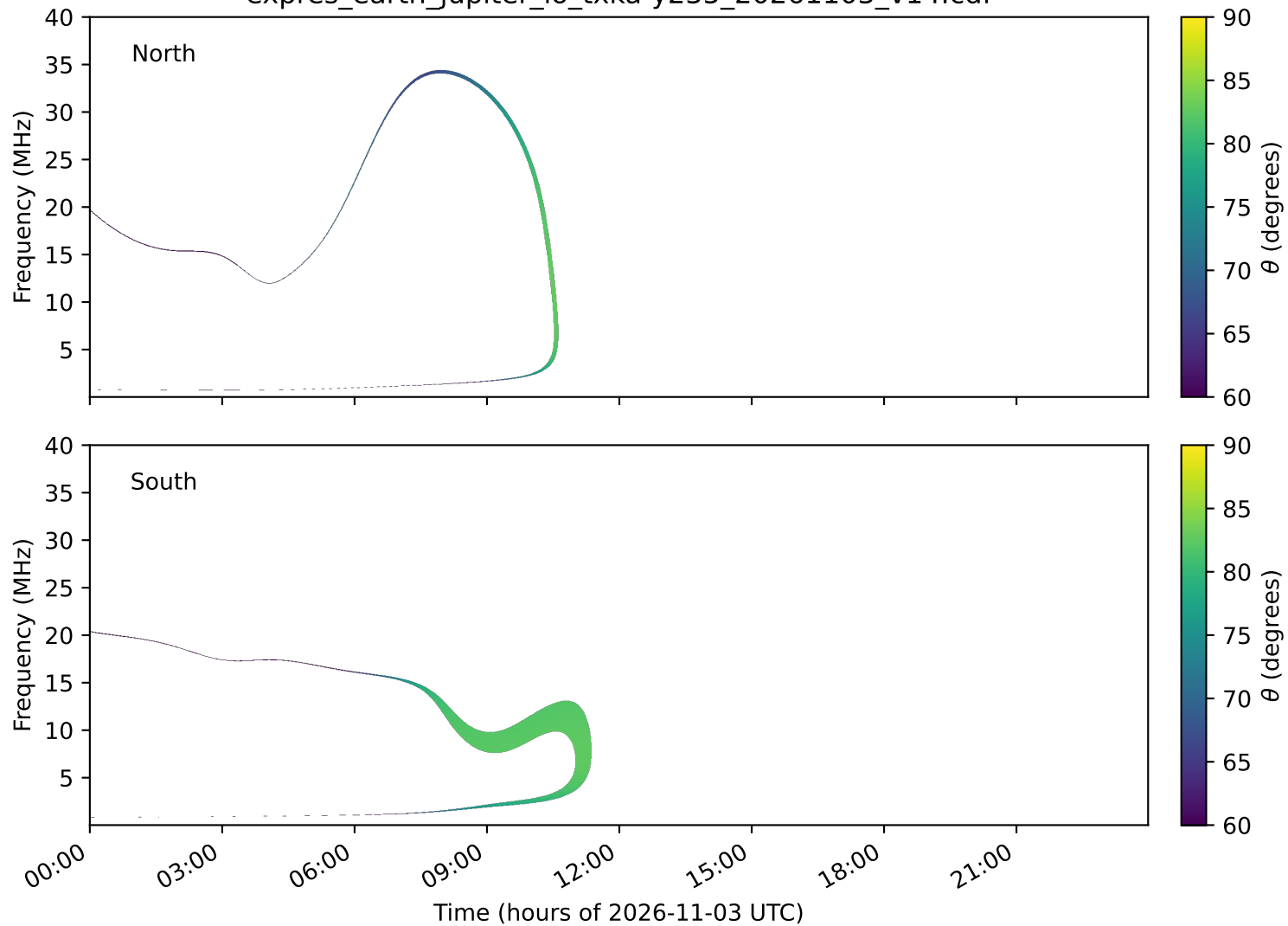
expres_earth_jupiter_io_txka-y235_20261103_v14.cdf
