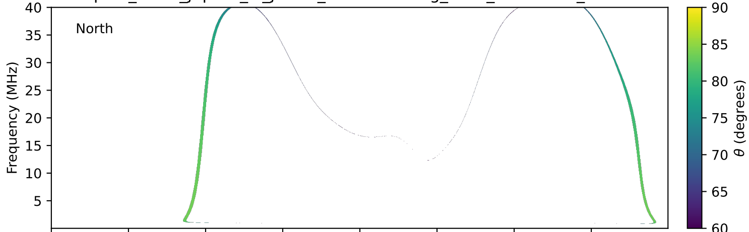
expres_earth_jupiter_io_jrm33_lossc-wid1deg_3kev_20261129_v11.cdf
