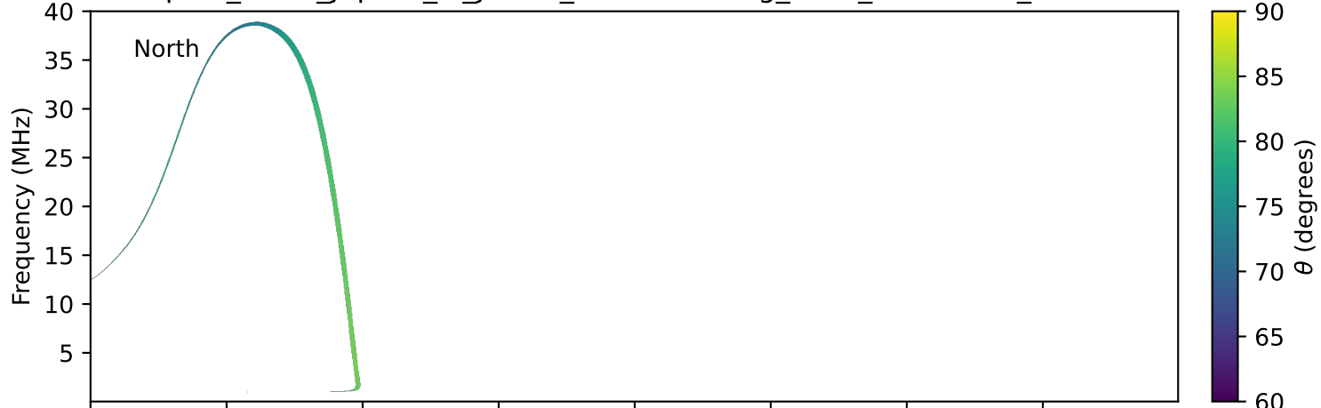
expres_earth_jupiter_io_jrm33_lossc-wid1deg_3kev_20261128_v11.cdf
