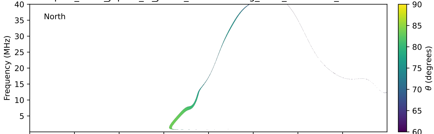
expres_earth_jupiter_io_jrm33_lossc-wid1deg_3kev_20261127_v11.cdf
