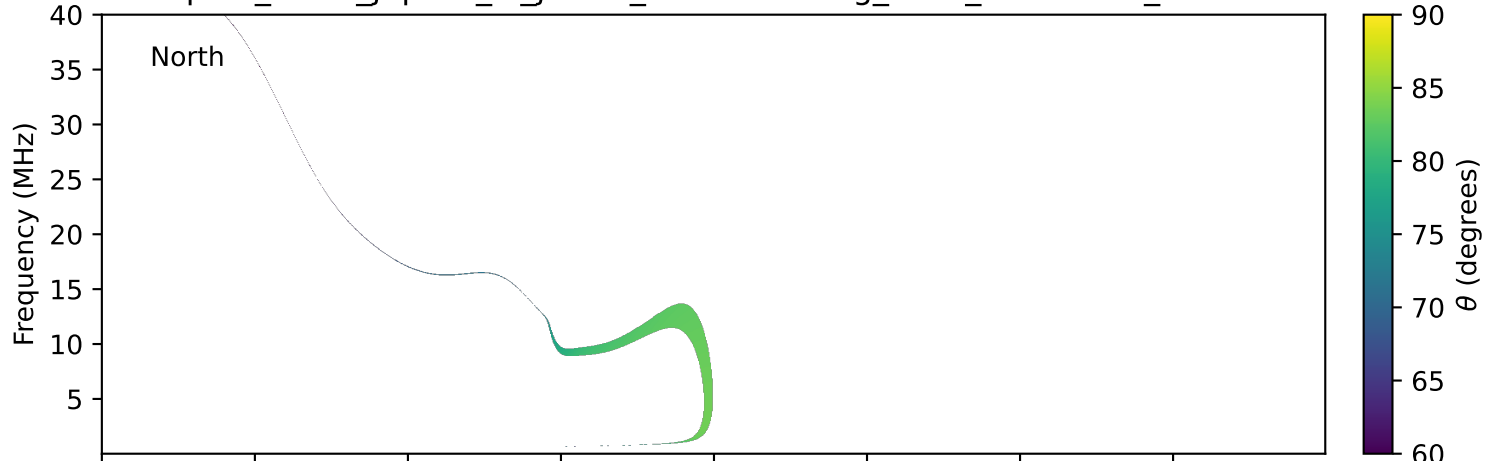
expres_earth_jupiter_io_jrm33_lossc-wid1deg_3kev_20261126_v11.cdf
