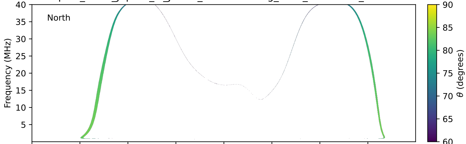
expres_earth_jupiter_io_jrm33_lossc-wid1deg_3kev_20261122_v11.cdf
